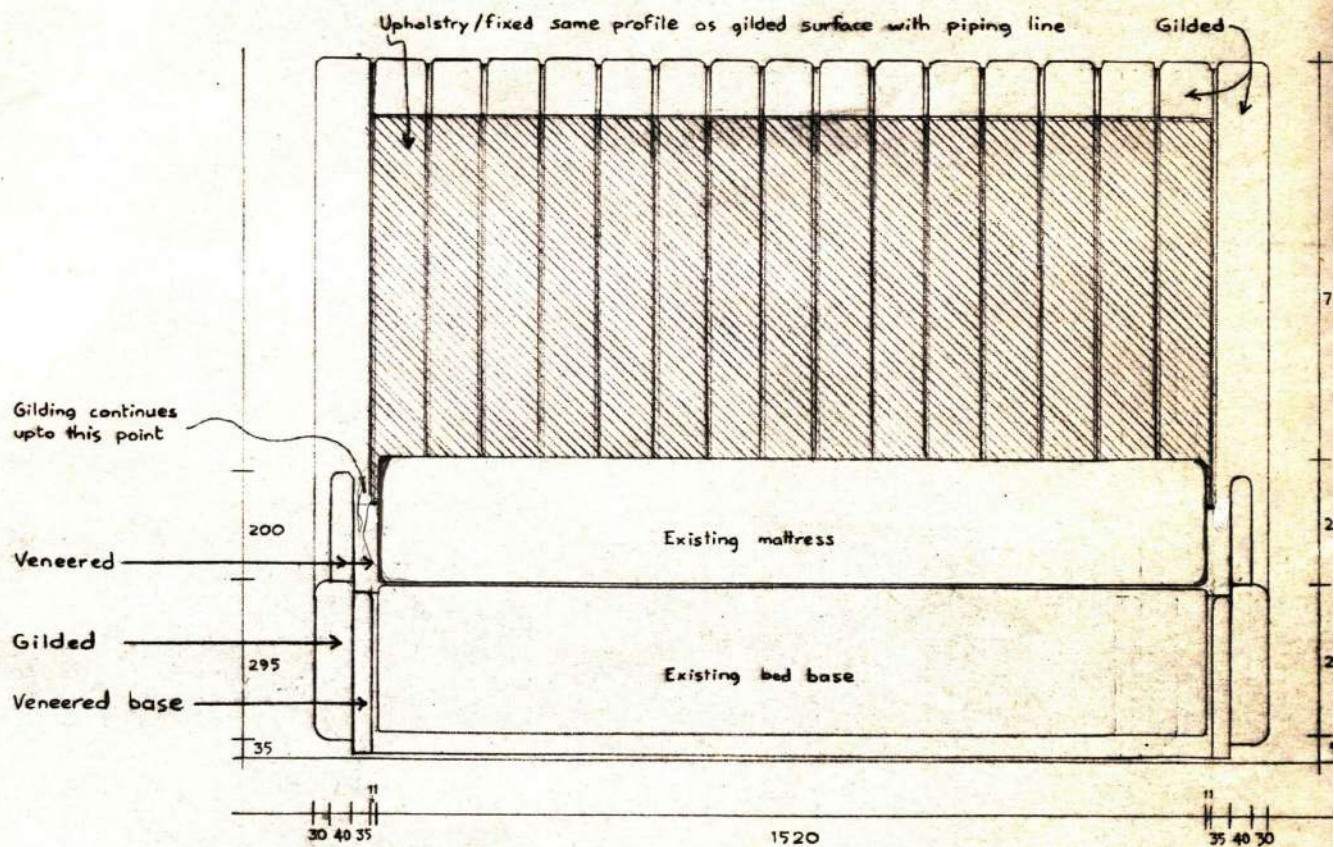
SECTION EE
