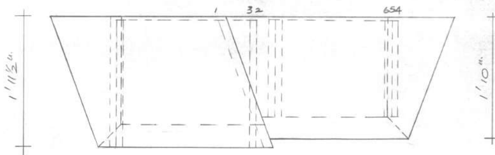
Drawers 1-3 Drawers 4-6 FRONT ELEVATION
