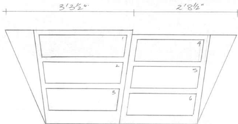
Drawers 1-3 Drawers 4-6 FRONT ELEVATION
