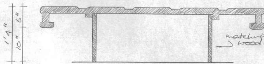
SECTION
