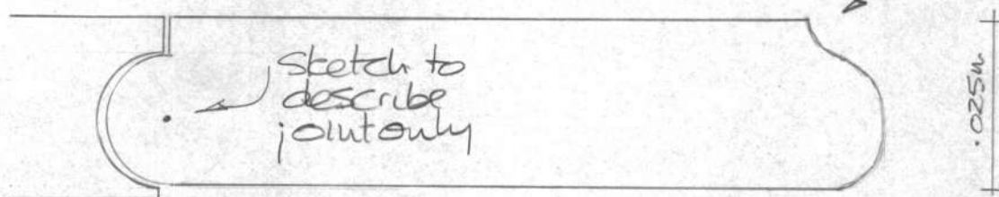
Full Scale Showing Flap Detail + Edge Profile
