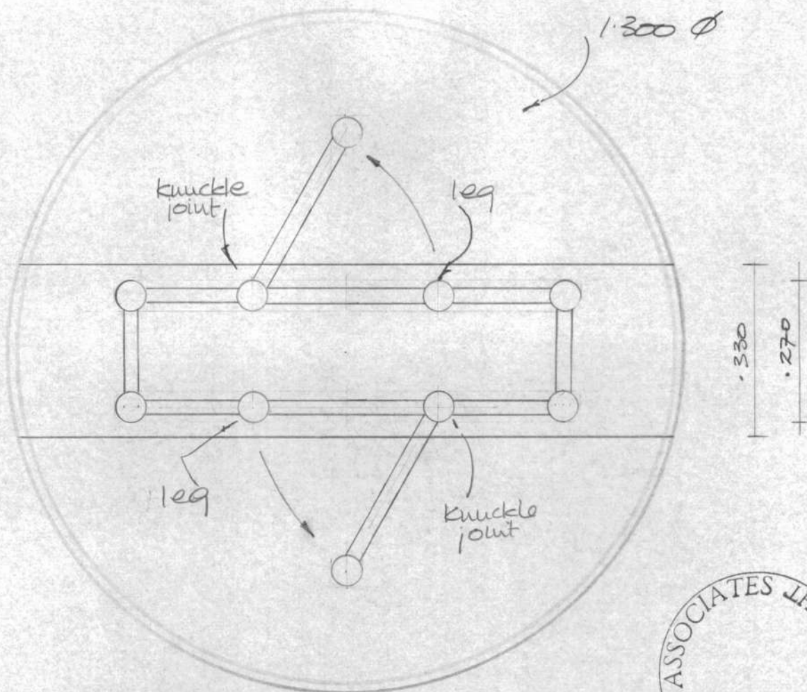
PLAN / PLAN SECTION showing flaps raised / legs extended.
