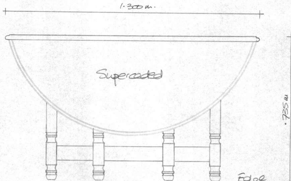
Long Side Elevation - Flap Down
